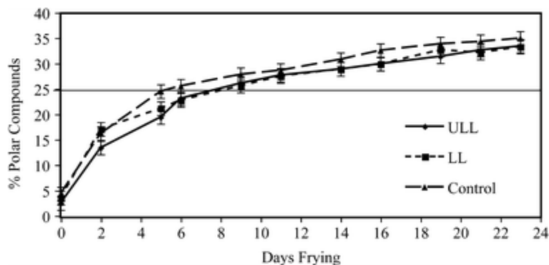
Fig. 2 Total polar compounds in ultra-low-linolenic acid (ULL), low-linolenic acid (LL) and control soybean oils throughout frying. Each value represents the mean of two replications. Bars around each data point indicate standard error of the mean for all data points. The value of 25% polar compounds is used in some countries as the maximum allowed, i.e. the discard value for frying oils [17]
